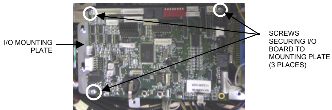
FIGURE 4 - I/O BOARD AND MOUNTING PLATE
