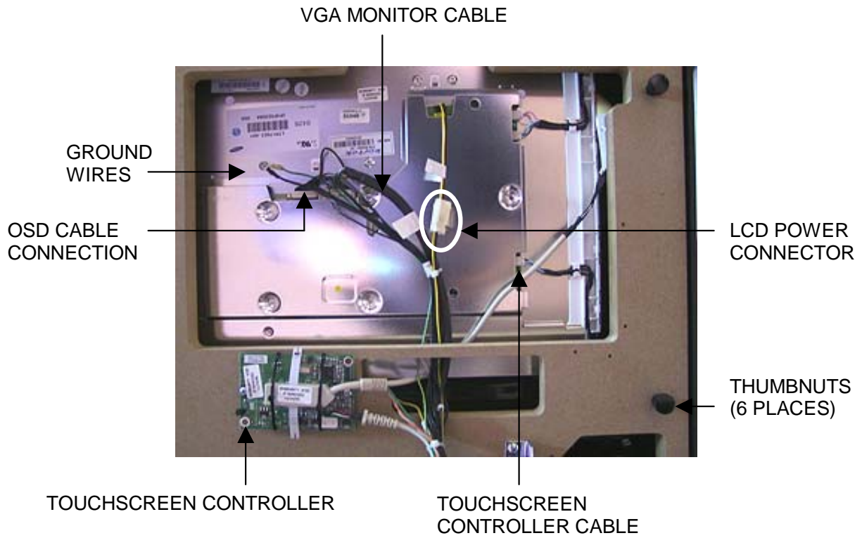
FIGURE 1 - REAR VIEW OF MONITOR / UNDERSIDE OF BEZEL
