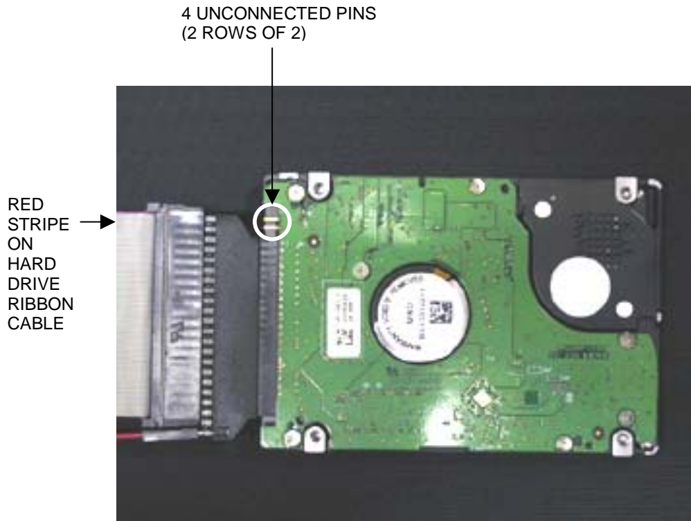
FIGURE 2 - CIRCUIT-BOARD SIDE OF HARD DRIVE
