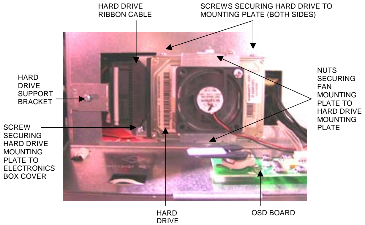
FIGURE 1 - HARD DRIVE ASSEMBLY ON ELECTRONICS BOX
