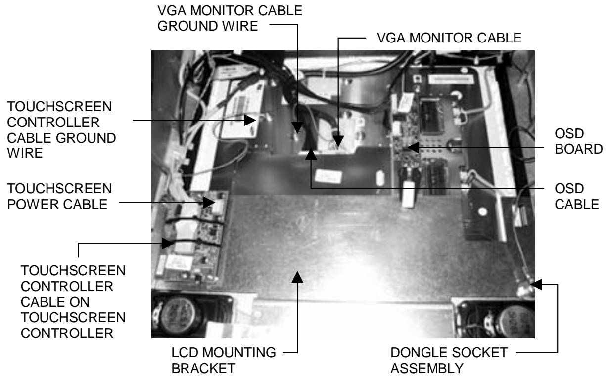
FIGURE 1 - CLOSEUP OF CPU SECTION
