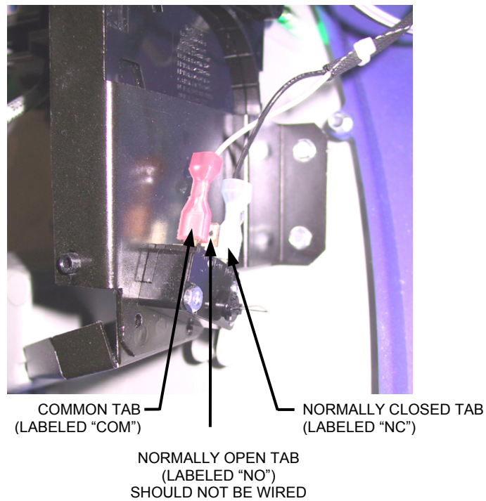
FIGURE 1 – CORRECT WIRING OF MOD BOX COIN MECH
