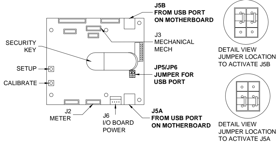
FIGURE 31 - I/O BOARD DRAWING
