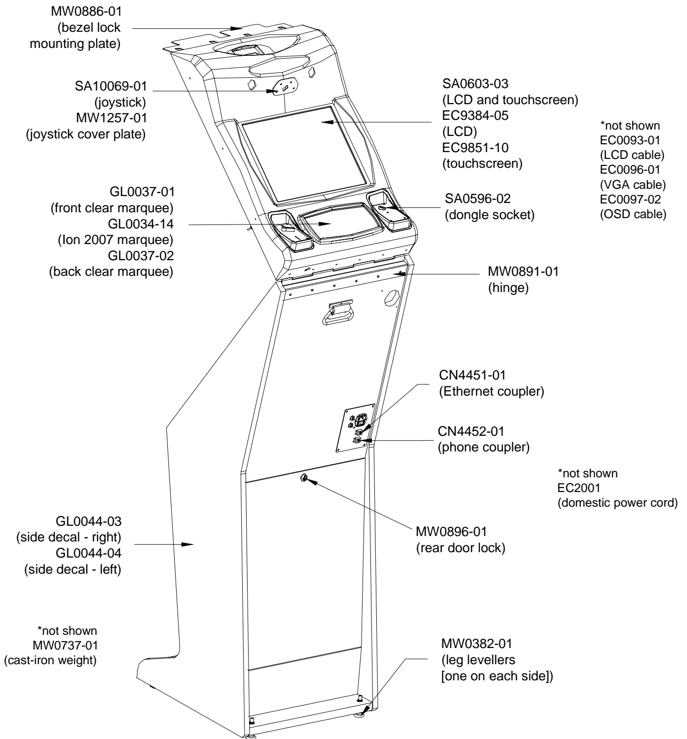
REAR VIEW OF THE FUSION WITH THE BEZEL OPEN
