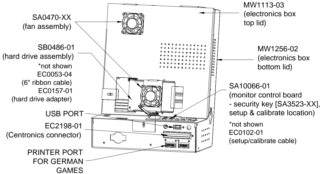
DETAIL VIEW OF ELECTRONICS BOX WITH COVER ON
