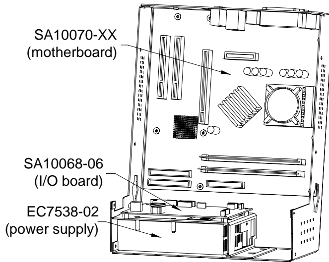
DETAIL VIEW OF ELECTRONICS BOX WITH COVER REMOVED
